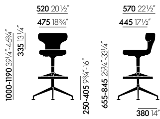
Pivot Counter Stool
