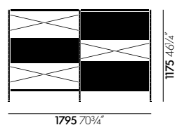
ESU Shelf, 3 UH
